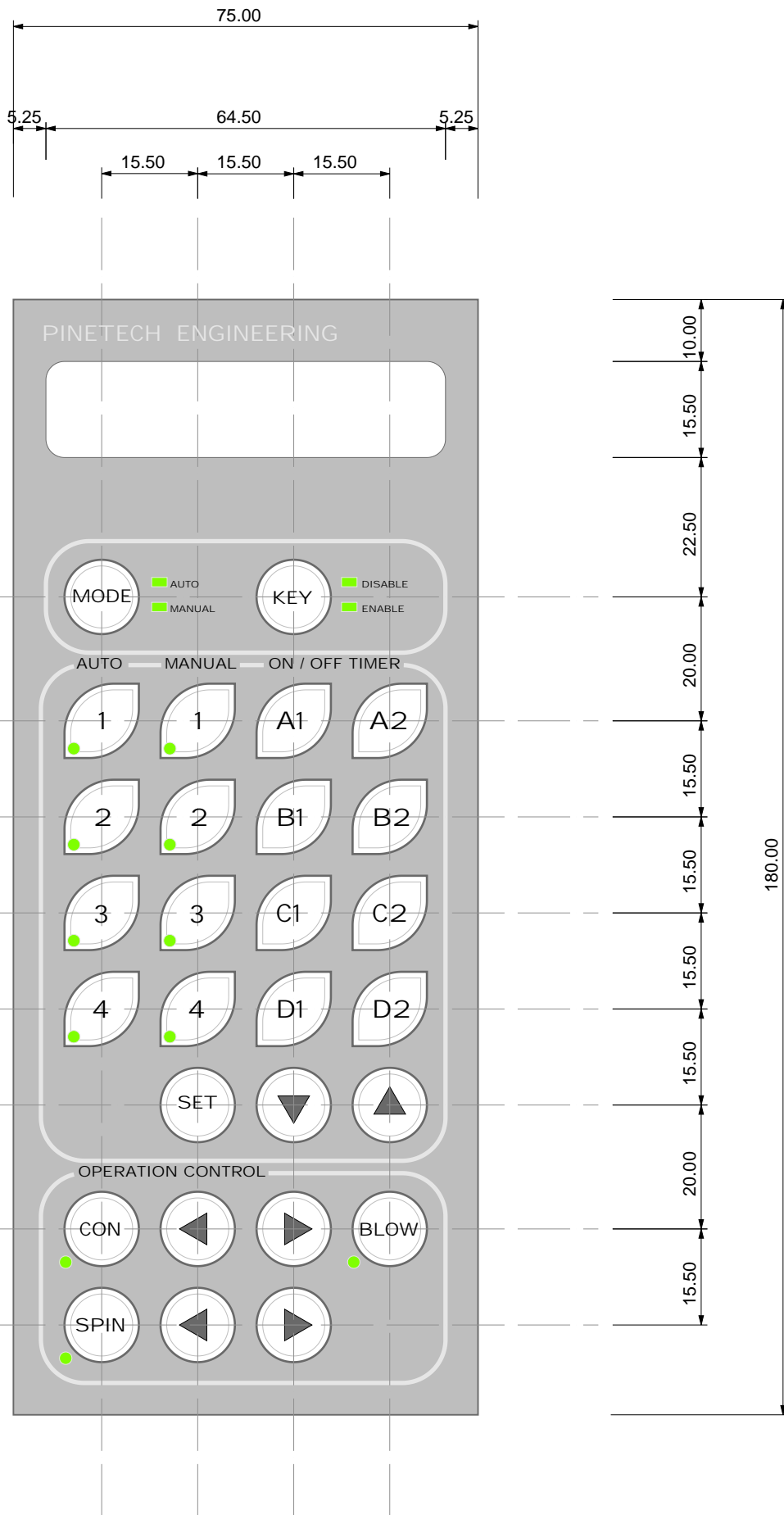
CONTROL PANEL LAYOUT SCALE 1:1 @ A4
